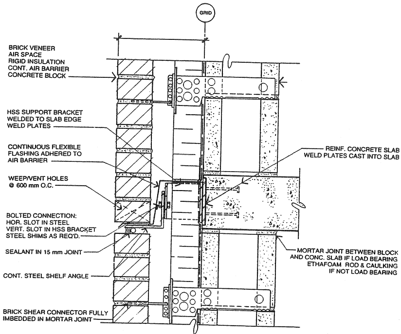
Figure 2 Brick Veneer/Concrete Block Detail At Slab Edge
