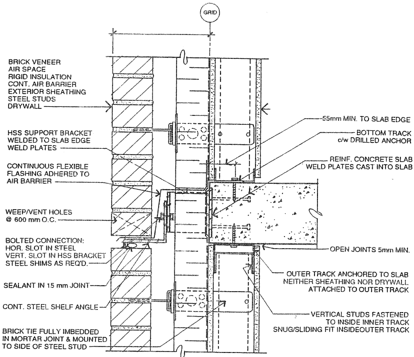
Figure 1. Brick Veneer/Steel Stud Detail At Slab Edge
