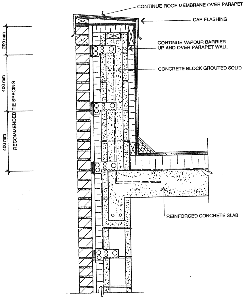
Figure 4. Brick Veneer/Concrete Block Detail At High Parapet
