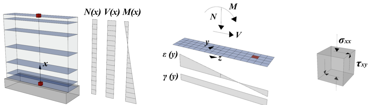
Figure 1: Formulation of the force-based beam element with coupling between axial and shear stress
