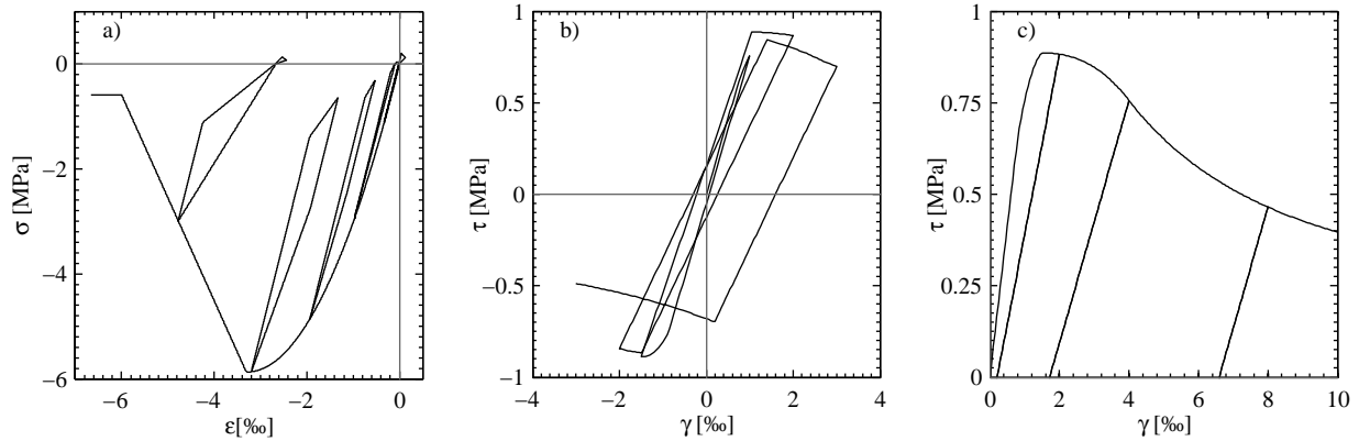
Figure 3: Cyclic behaviour of the material model in compression (a) and shear, under a constant axial load (b, c). Main material properties: f_c = 5.7 MPa, f_t = 0.25 MPa, c = 0.25 MPa, \tan \phi_{in} = 0.4 , \tan \phi_{fn} = 0.2 , G_f^c = 8 N/mm, G_f^I = 0.05 N/mm, G_f^{II} = 0.5 N/mm
