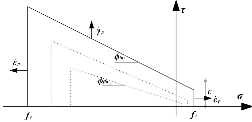
Figure 2: Yield domain of the material model
