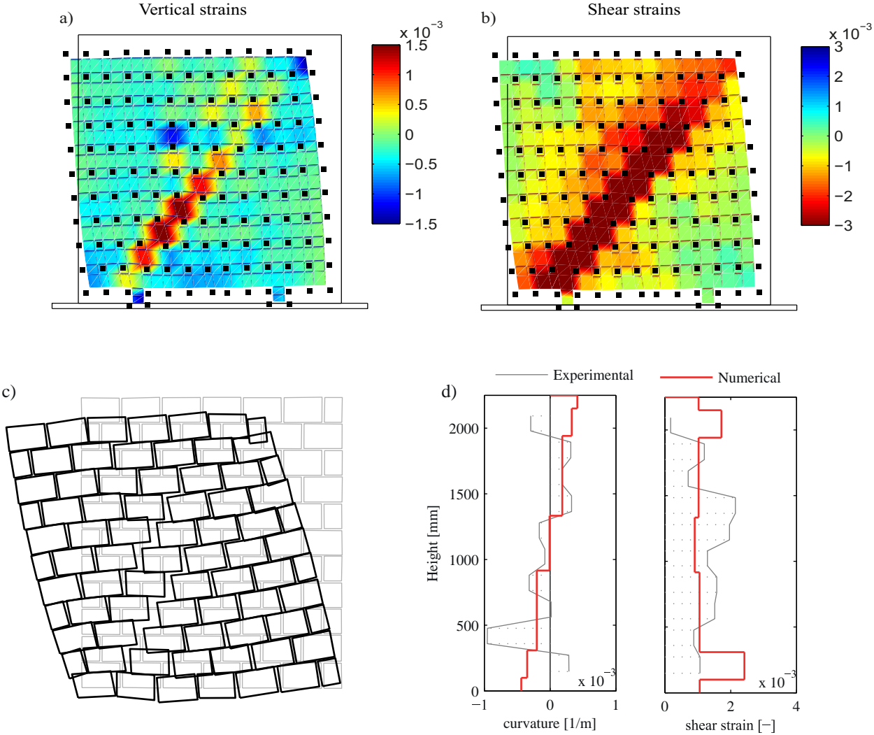
Figure 6: Local experimental deformation fields: vertical strains, (a) and shear strains (b). Deformed displacement field with warping of the sections due to shear (c). Comparison of experimental and numerical curvature and sectional shear deformation profiles (d)
