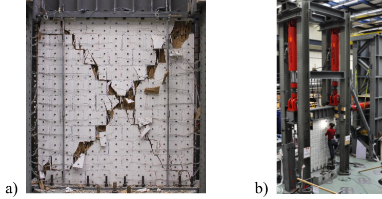
Figure 4: Wall PUP1 at failure (a), and test setup, showing the position of the three red actuators (b) [18]
