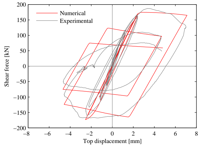
Figure 5: Comparison between experimental results and numerical force-displacement response of the beam element
