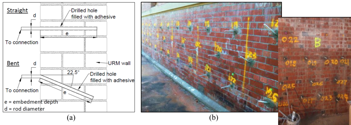
Figure 3: Testing arrangement of adhesive anchors: a) Test parameters; b) Wards Brewery Building 2, Christchurch; c) Phoenix Wine and Spirits Building, Whanganui.
