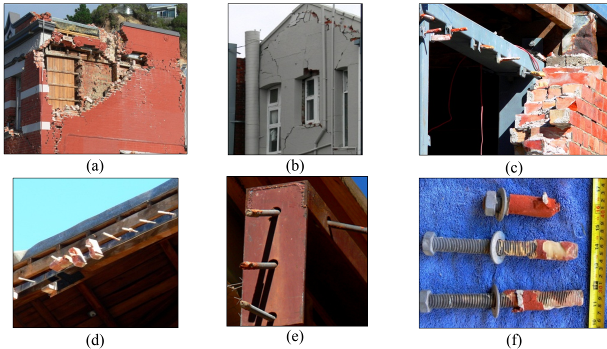
Figure 1: Wall-to-diaphragm anchors: a) Row of successful wall-to-diaphragm anchors, with wall failure beneath; b) Failure of the gable due to low shear strength of masonry, despite sufficient anchorage; c) Insufficient embedment depth of adhesive anchors; d) Large number of adhesive anchors unsuccessful at preventing out-of-plane collapse of URM wall; e) Insufficient adhesive used only at the tip of anchors; f) Recovered adhesive anchors that performed inadequately.
