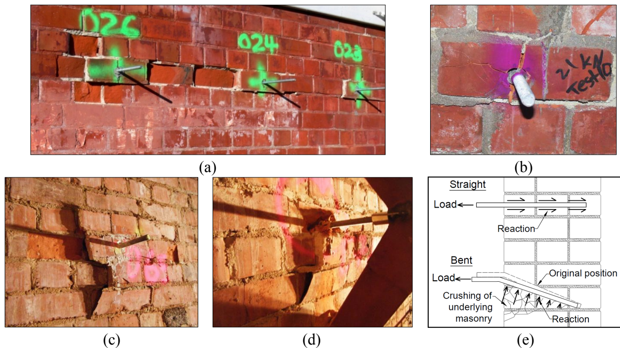
Figure 6: Typical failure modes: a) Typical masonry pull-out type failure observed; b) Localised splitting of brick; c) Straight anchors; d) Bent anchors; e) Schematic view of observed failure modes.
