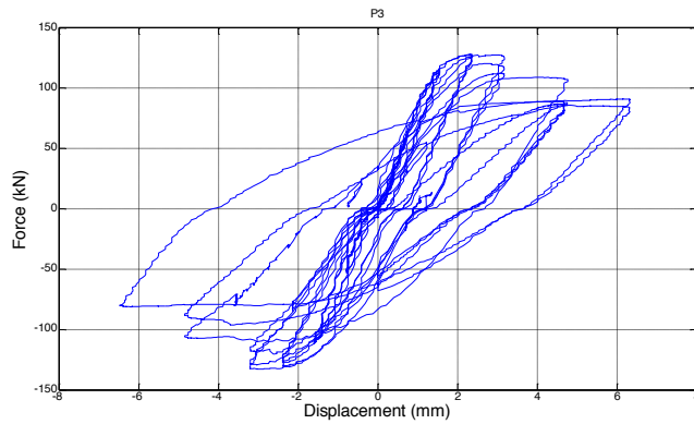
Figure 6: Hysteretic Response of Wall P3
