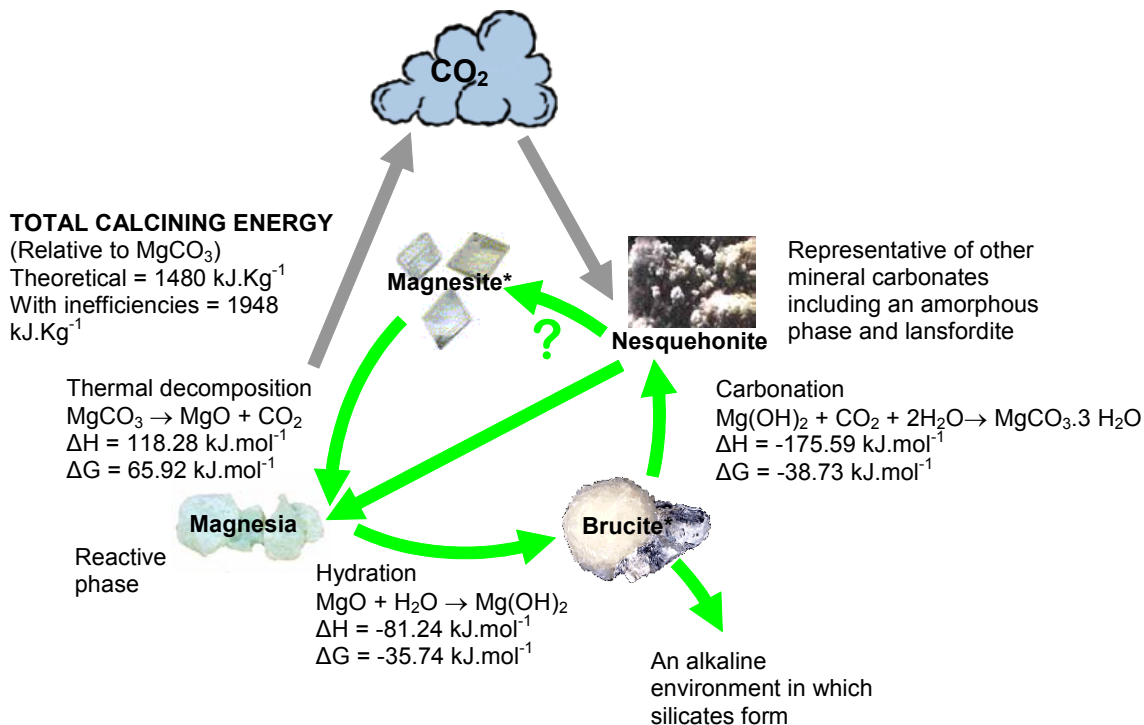
Figure 1 - The Magnesium Thermodynamic Cycle
