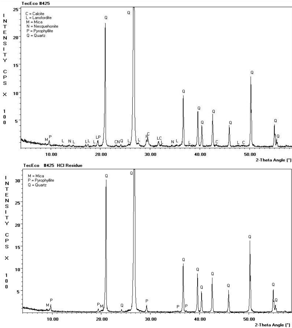
Figure 2 - XRD Showing Carbonates Before and Minerals Remaining after their Removal with HCl in a Simple Mix (70 kg PC, 70 kg MgO, colouring oxide .5kg, sand unwashed 1105 kg)
