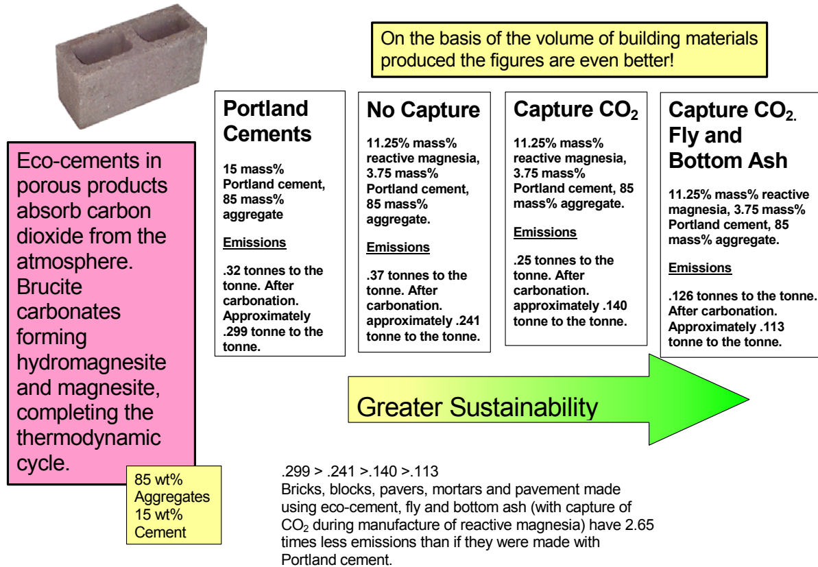
Figure 3 - The Carbonation of a Typical Eco-Cement Block
