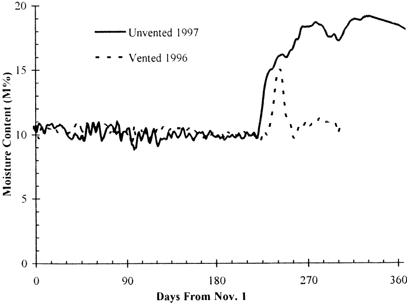
Figure 5: Framing Moisture Content Vs Time
