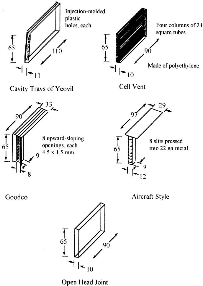
Figure 2: Head Joint Vent and Vent Inserts Tested
