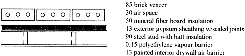
Figure 4: Simplified Test Panel Cross Section
